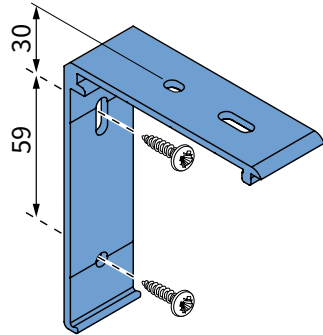
Wandmontage
